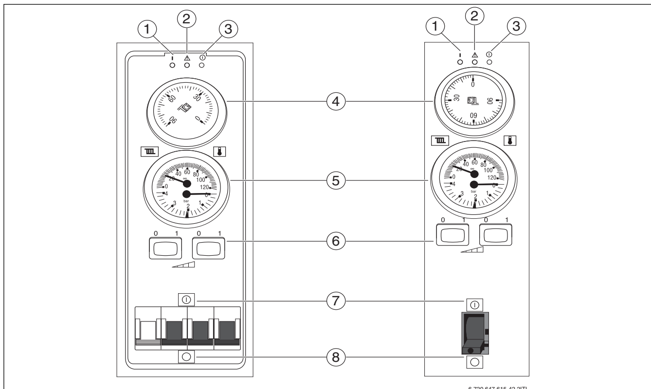
Obr. 2 Obslužný panel Tronic 5000H
