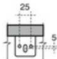
Part section through basin on E5010 hangers
