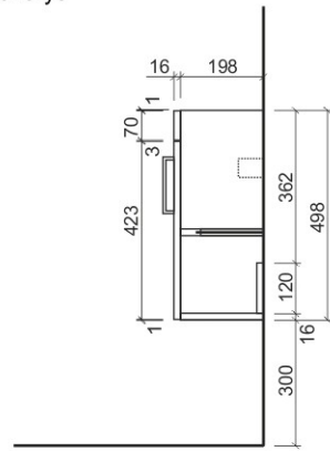
Bokorys
