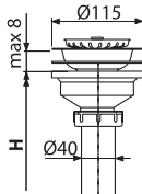
A446: H=120-225 A446P: H=165-225
