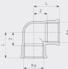
Oblouk 90° - mosaz model 1612
