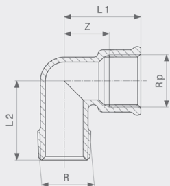
Koleno 90° - mosaz model 1613
