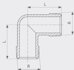
Koleno 90° - mosaz model 1611
