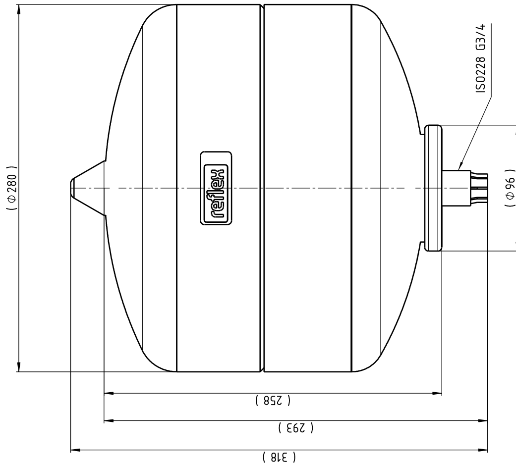
Front view
